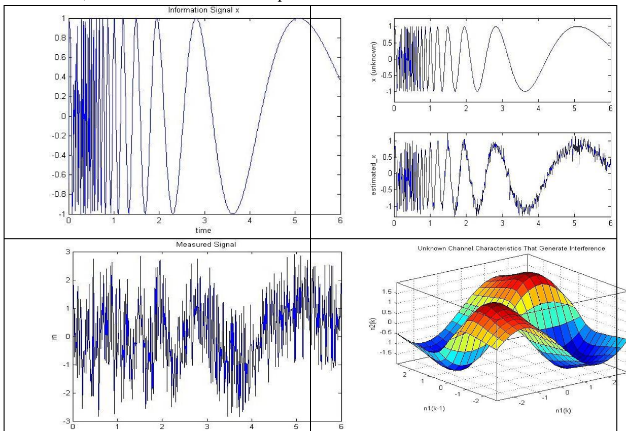
Figure 2. Measured signal
