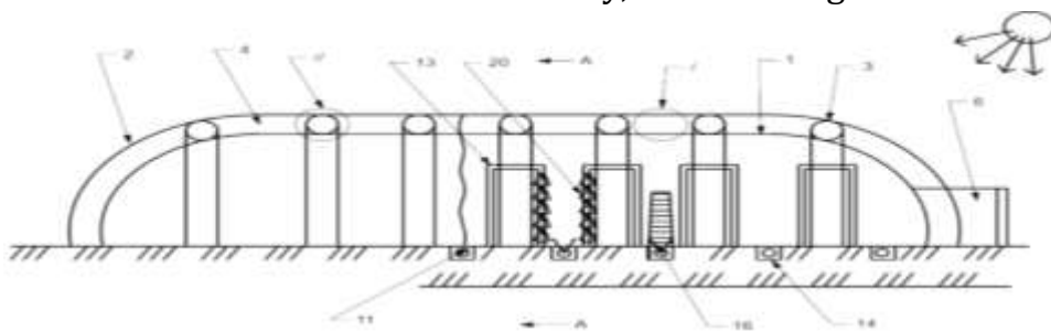
Fig.1. Double-layer pneumatic structure as a solar-radiation drying plant for drying grapes
